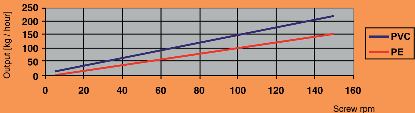
Extrusion output for TEA 70.25
